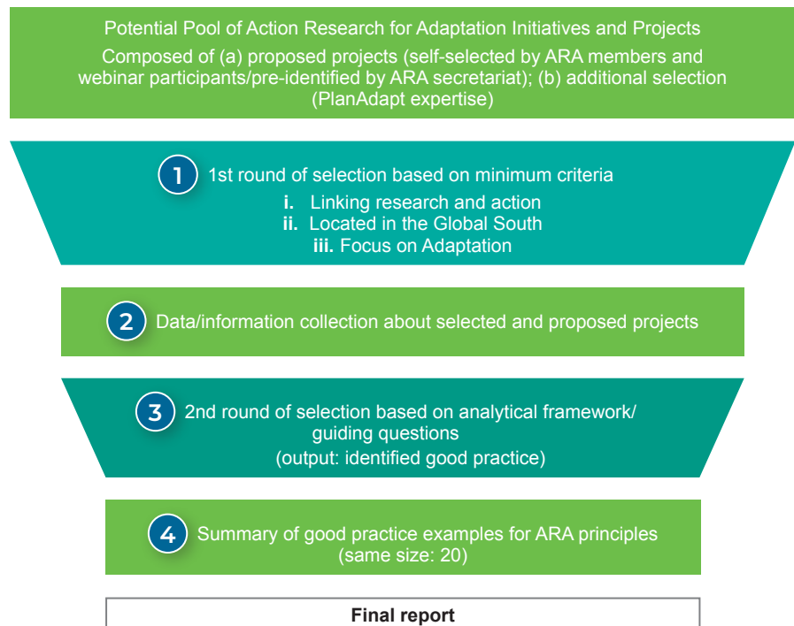
FIGURE 5: Analytical framework
